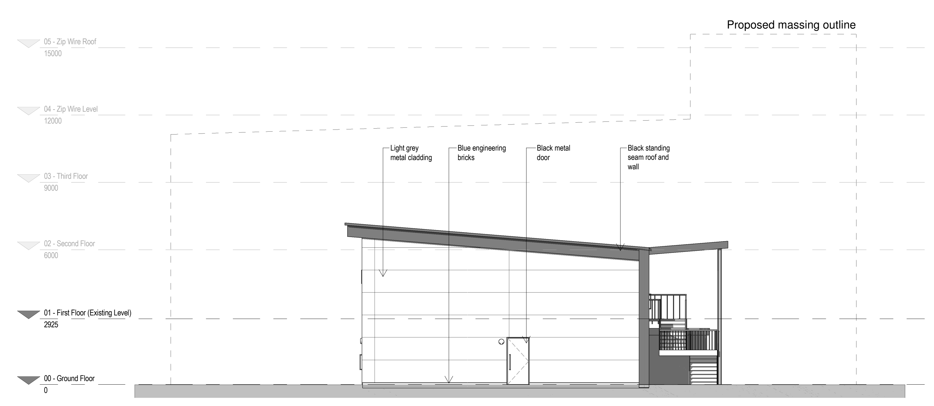
Existing Elevation 3
